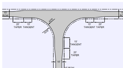
Figure 3-5: Alley-to-Alley Intersection
