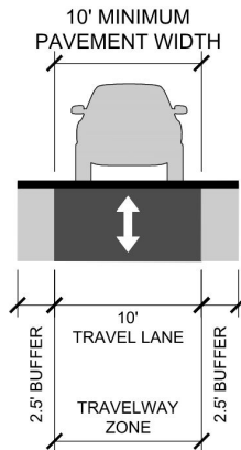
Figure 3-1: Alley Typical Section Land Use Context: Neighborhood
