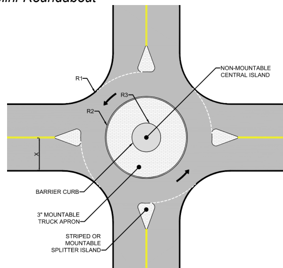
Figure 13-9: Mini-Roundabout
