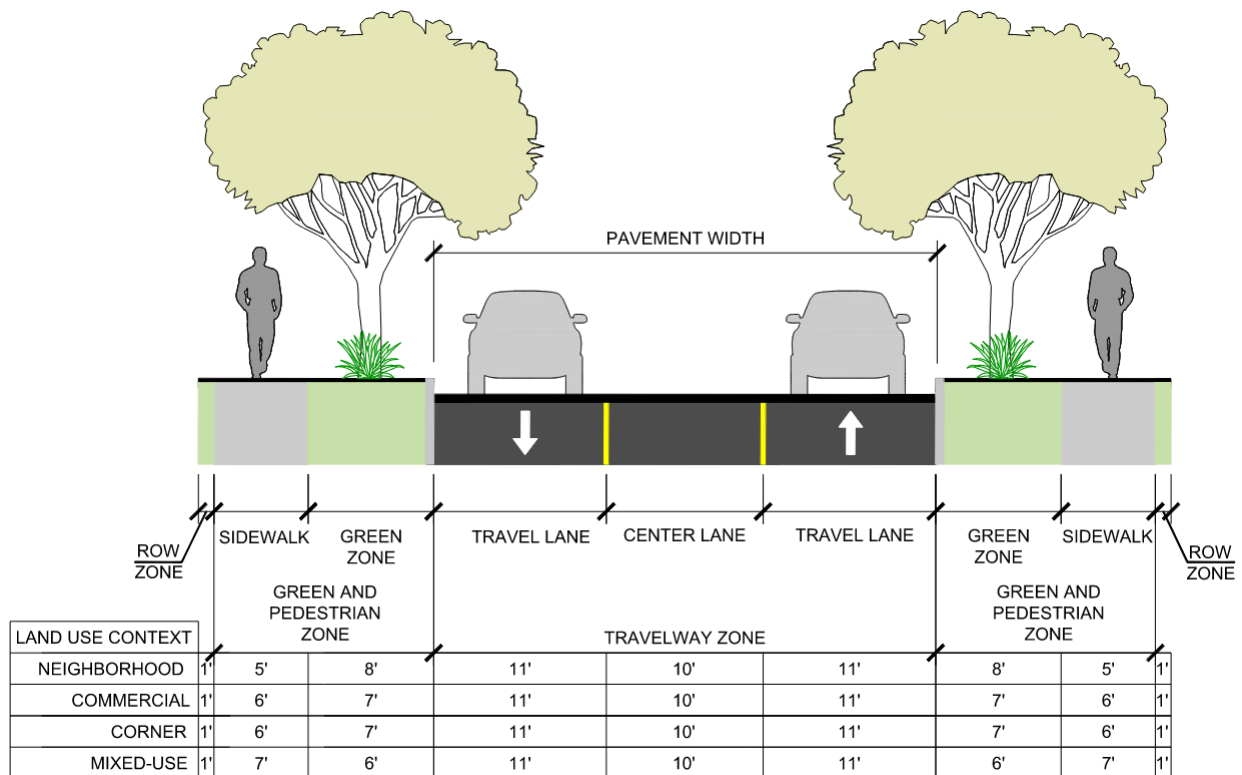
Figure 2-19: Type F Special Condition (Center Turn Lane) – 60' ROW
