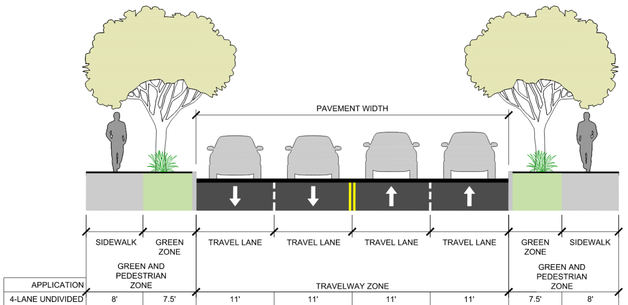
Figure 4-14: 14th Street – Municipal Avenue to P Avenue (75' ROW) Option C
