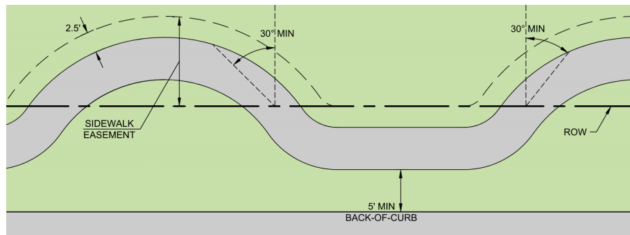
Figure 9-4: Meandering Sidewalk
