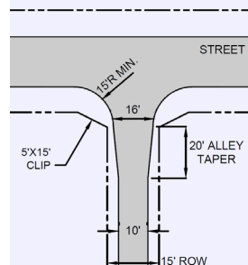
Figure 3-6: Alley-to-Street Intersection
