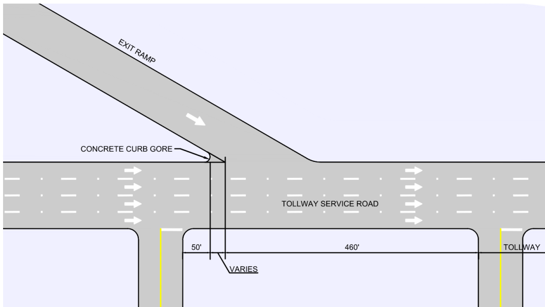
Figure 5-12: Dallas North Tollway Access Standards (Crossing Thoroughfare Drive Spacing, applicable to other Tollways)
