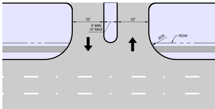
Figure 8-4: Driveway Width, Radius, and Spacing for Divided Commercial and Industrial Driveways
