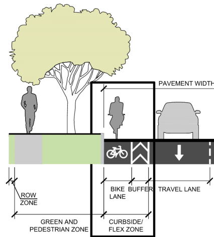
Figure 9-7: Buffered Bike Lane
