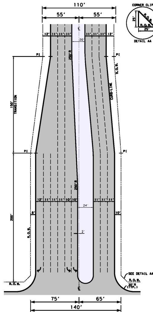
Figure 6-3: Intersection of Type C with Tollway Service Road, ROW Requirements
