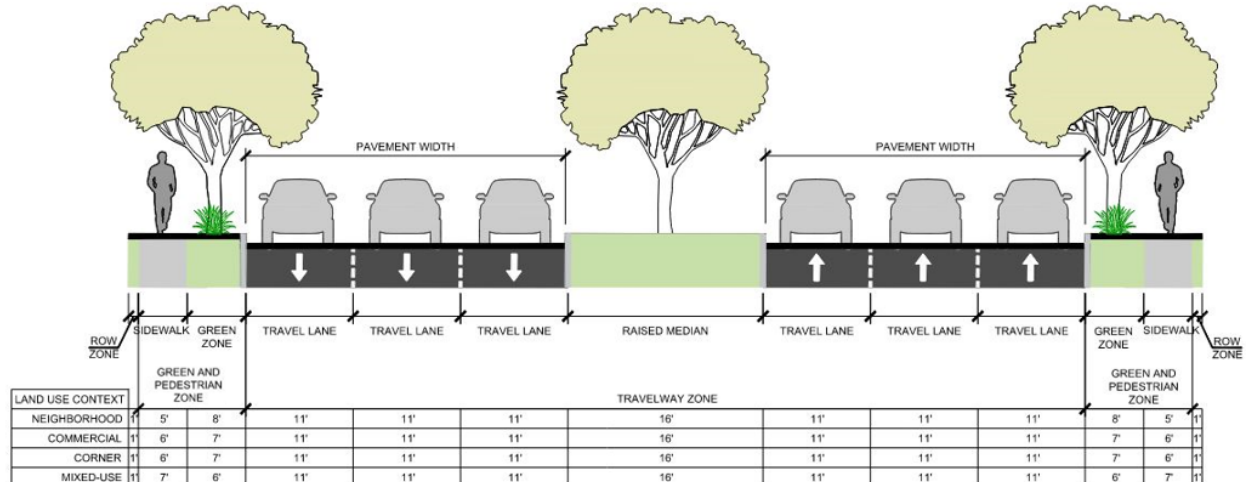
Figure 2-5: Type C Typical Section – 110' ROW
