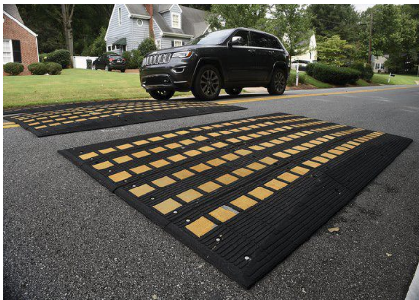
Figure 13-13: Speed Cushions
