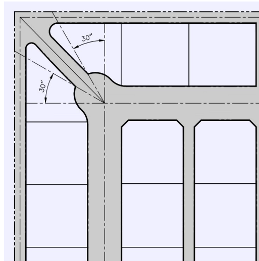
g. Figure 3-4: Alley Intersecting an Elbow
