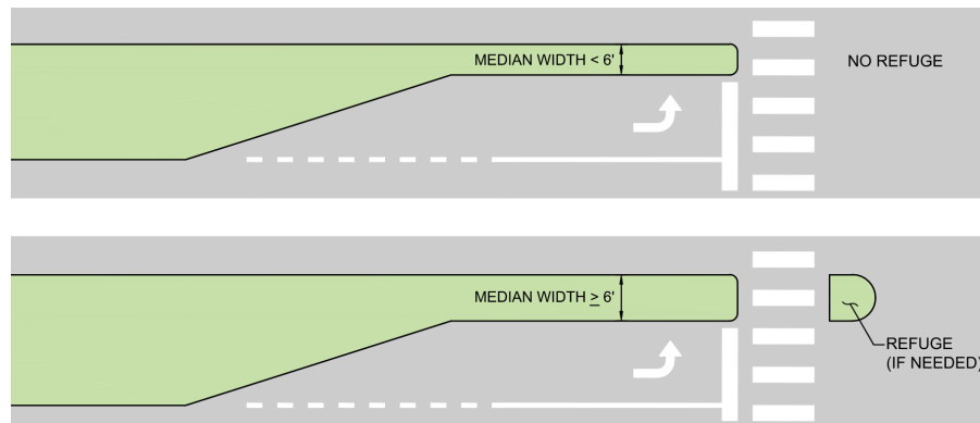
Figure 9-12: Crosswalk Refuge
