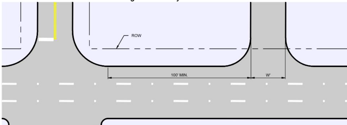
Figure 8-10: Driveway Spacing in Relation to a Cross Street - Driveway at 90° on a Regional or Major Arterial
